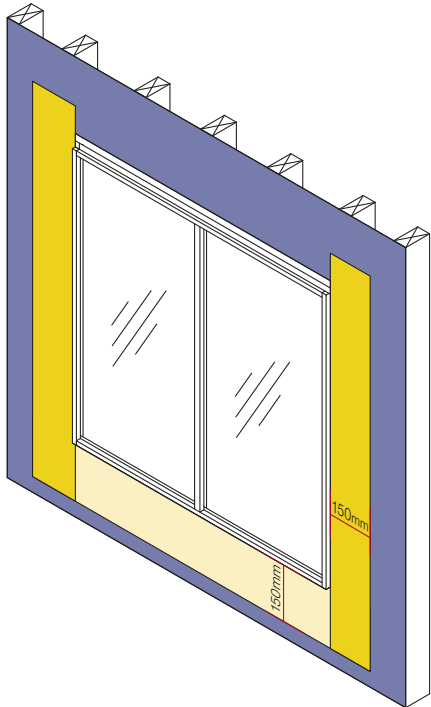
Figure 9 Jamb Flashing
